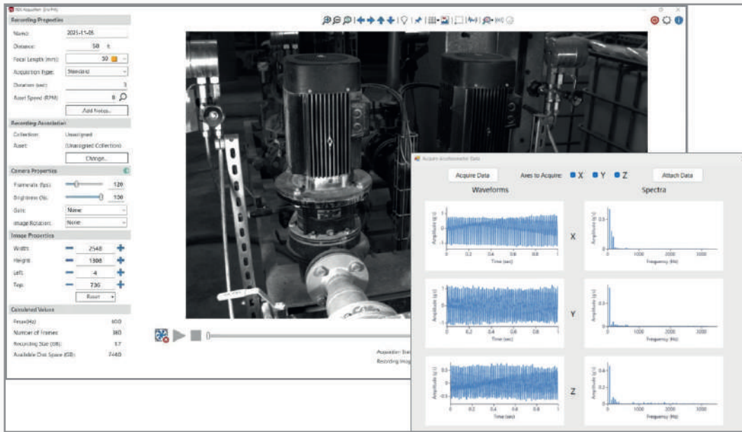
See bearing-level vibration and overall asset motion—simultaneously with TrueSight™ Accel.
